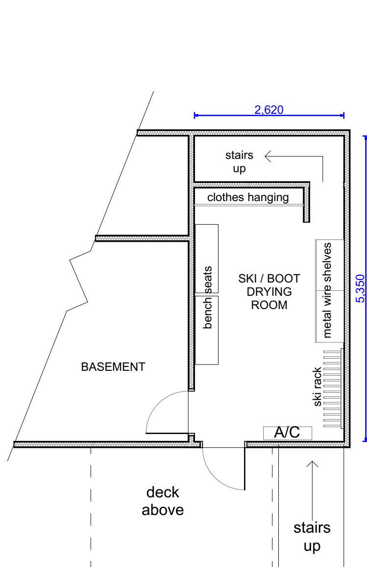
BOOT ROOM
